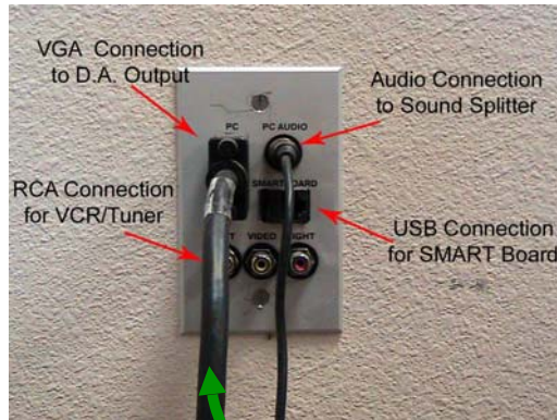
Wall Plate
